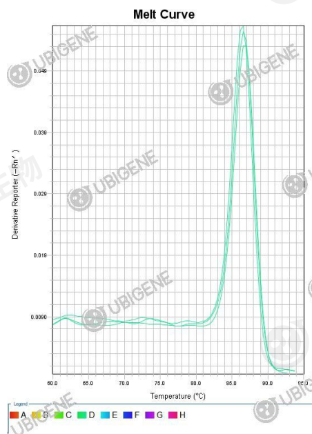
A549_Ctrl(Puro)+ \beta -h_actin melt curve
