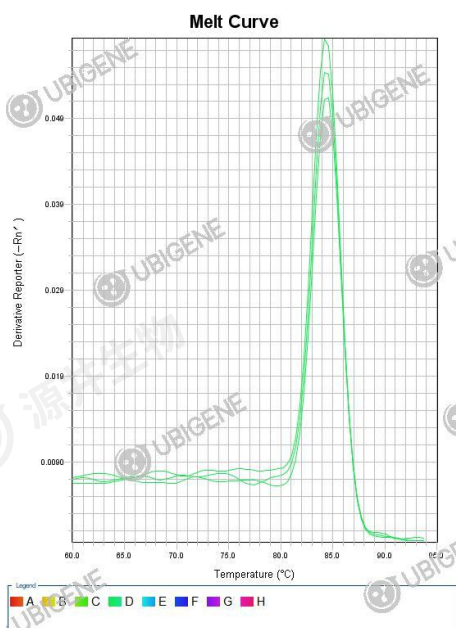
RPS6KA4 Stable Expression Cell Line (A549)+hRPS6KA4-1 melt curve
