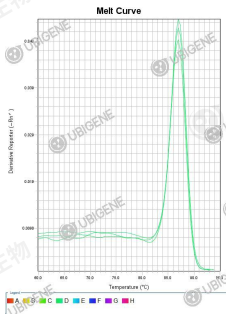
RPS6KA4 Stable Expression Cell Line (A549)+ \beta - h_actin melt curve
